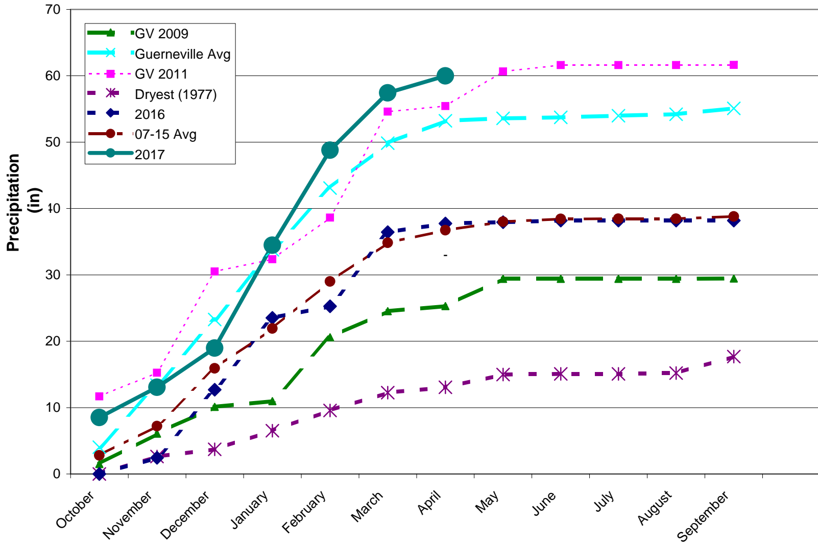
Figure 3. Guerneville Cumulative Monthly Rainfall
