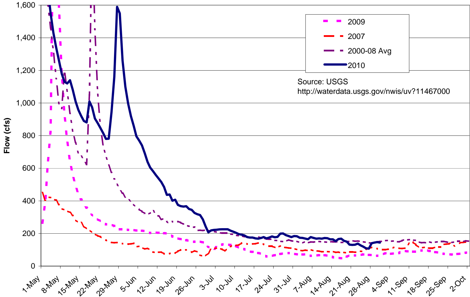
Figure 3. Russian River Summer Flow 2010 Hacienda Bridge, Updated August 27, 2010
